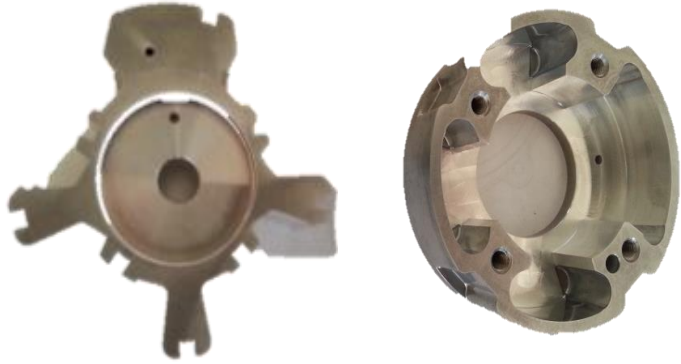
CVVT Rotor & Housing
